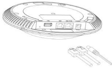
Figure 8: Connecting GWN AP - GWN7600 as example
