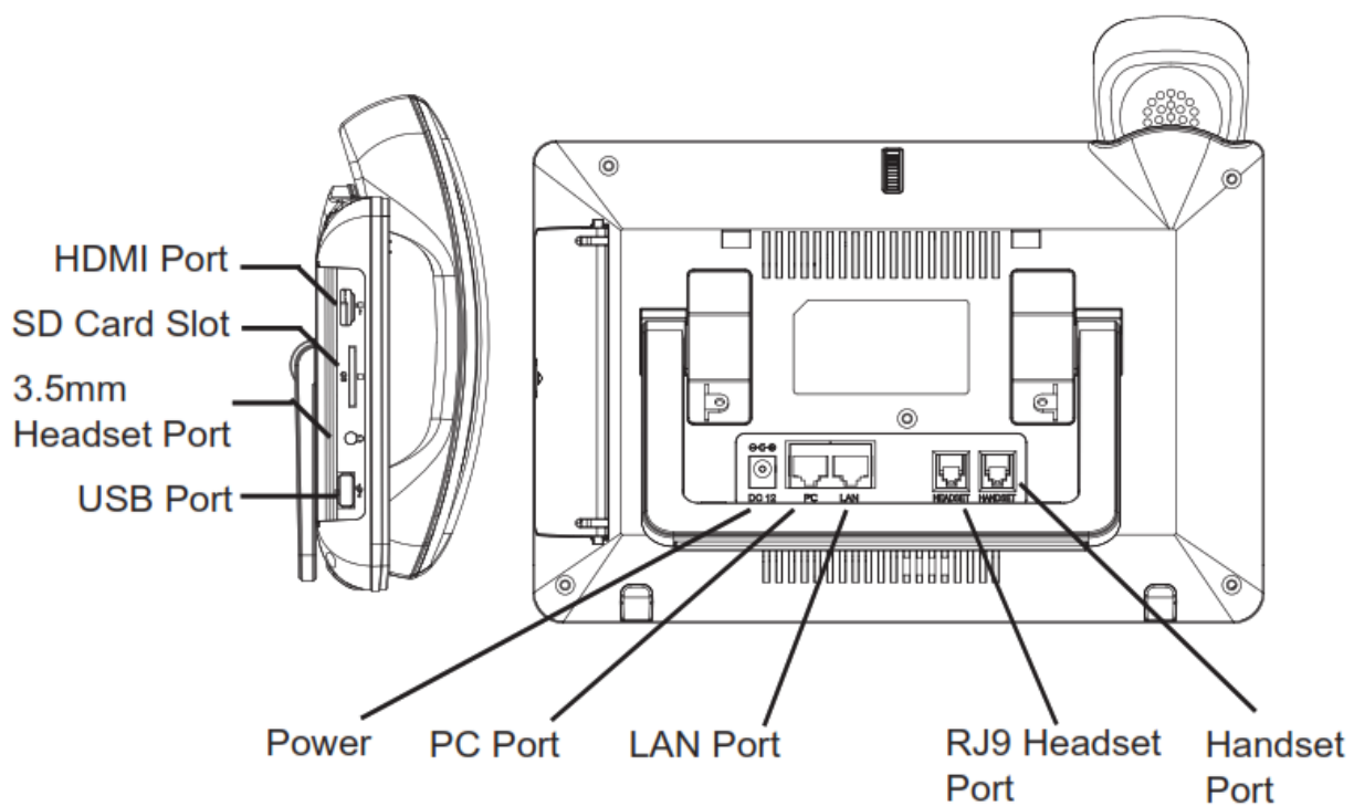
Figure 4: GXV 3370 Back / Side View
